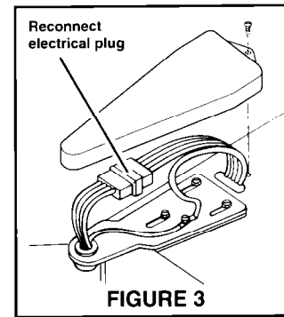
FIGURE 3 FREEZER DOOR ELECTRICAL PLUG
