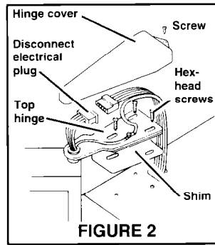
FIGURE 2 FREEZER DOOR TOP HINGE
